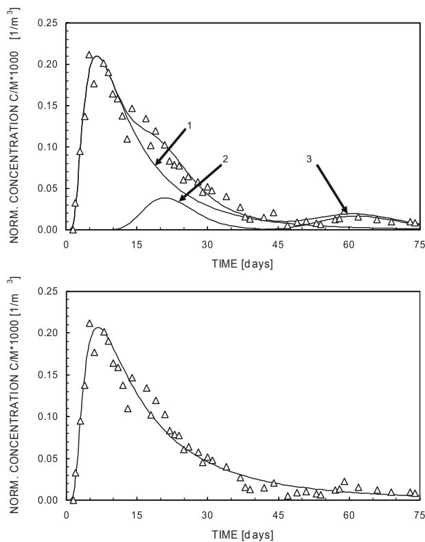
Fig. 4. The best fits of theoretical curves (heavy line) to the bromide concentrations (triangle) measured in the outflow from the pond ( C/M ) obtained by the calibration of the Multi-Flow Dispersion Model (upper) with three flow-paths (thin lines) and the Single-Flow Dispersion Model (lower). The concentrations ( C ) are normalized to the mass of tracer injected ( M ). The values of fitting parameters are summarized in Table 1.
