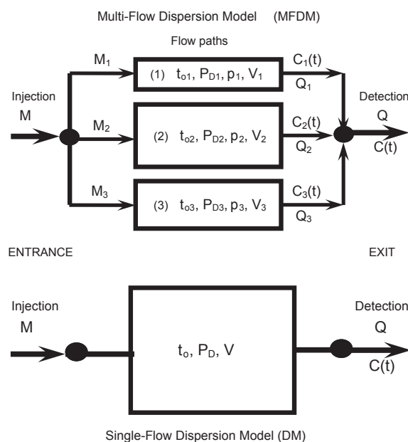
Fig. 3. The conceptual presentation of the Multi-Flow Dispersion Model (upper) and Single-Flow Dispersion Model (lower). Both models were applied for the modelling of bromide concentration curve measured during the tracer test.
